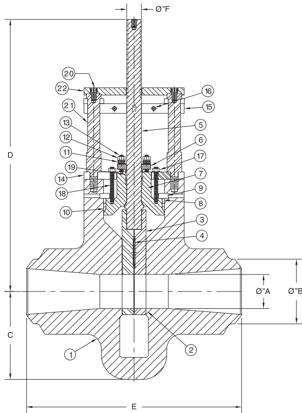
SECTION X-X
