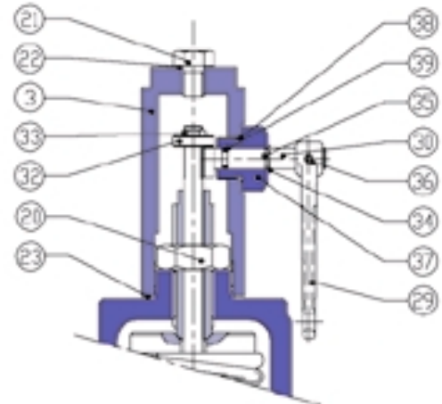
Packed Type F Lever (threaded)
