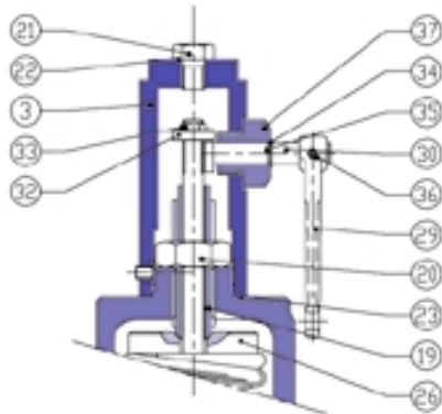
Plain Type C lever (threaded)
