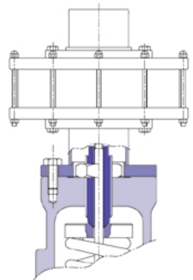
Pneumatic Actuator Type P
