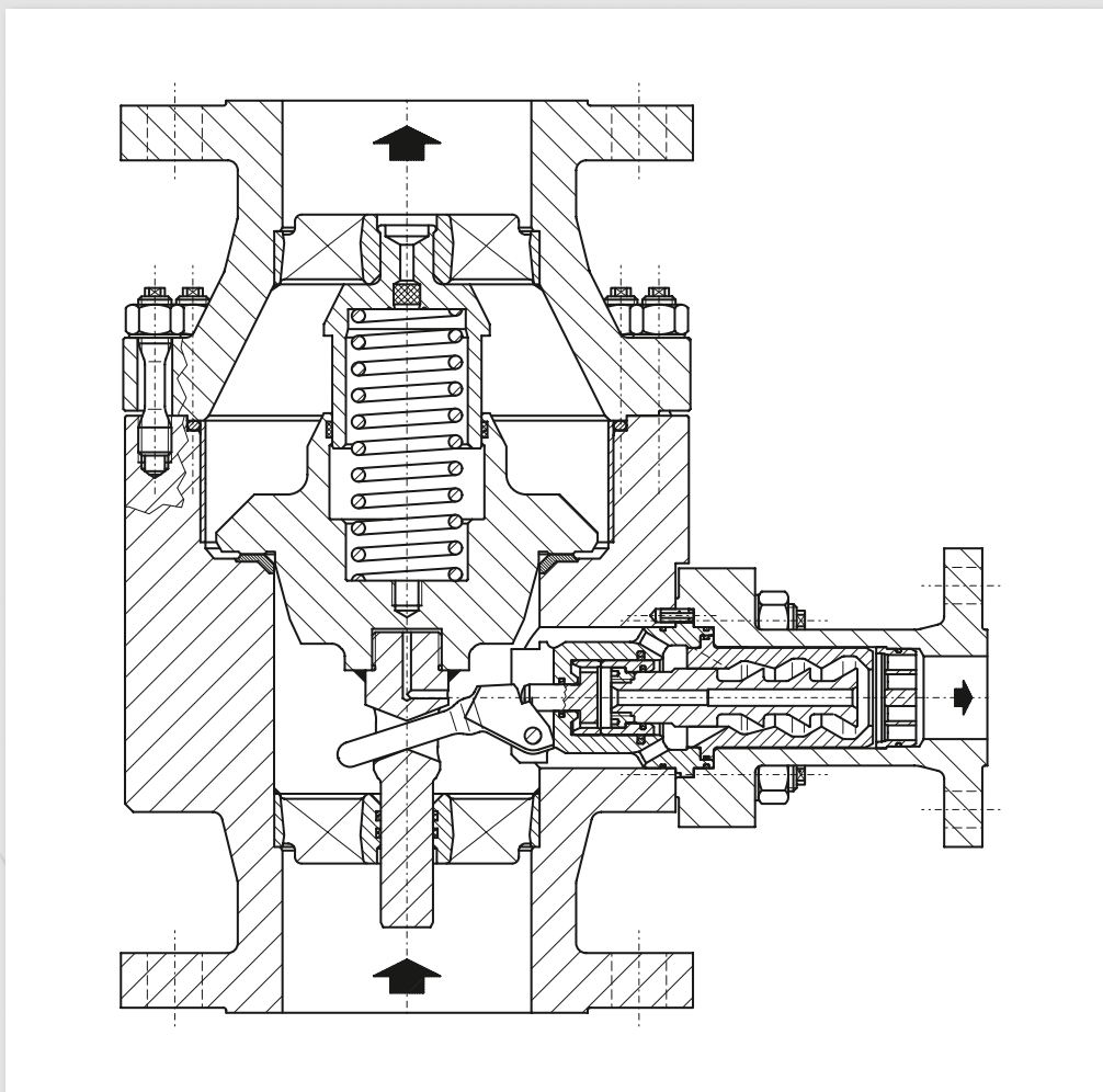
Fig.1: Drawing of an Automatic Recirculation Valve type TDM
