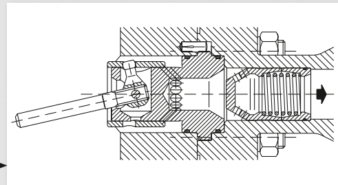
Fig. 4: Bypass M
