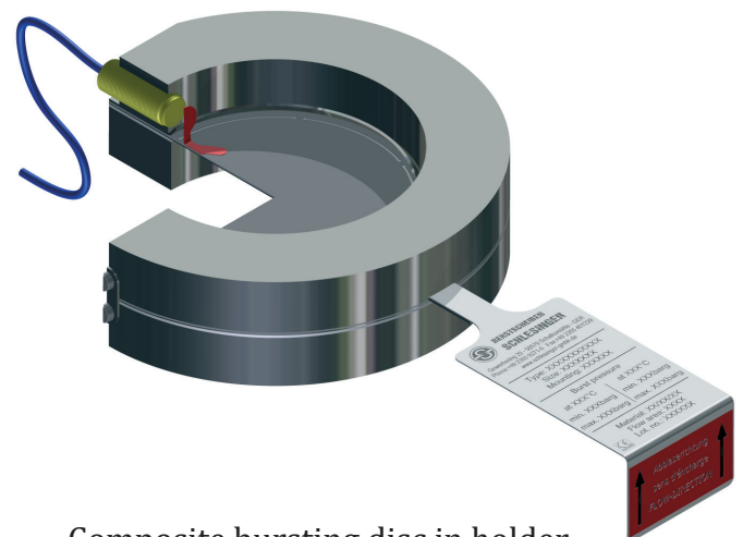
Composite bursting disc in holder with inductive signal detector
