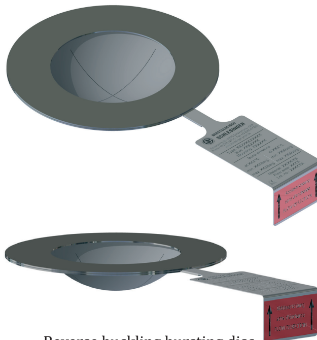
Reverse buckling bursting disc, Type UX (cross-scored)
