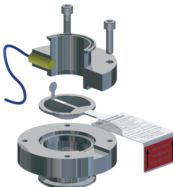
Reverse buckling bursting disc with inductive proximity switch in bursting disc holder Type BHS
